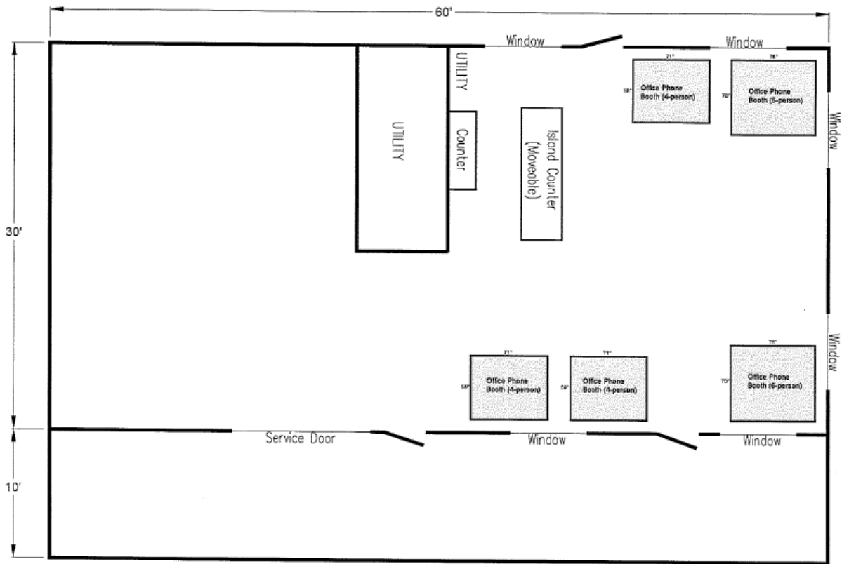
Tentative layout for three 4-person pods and two 6-person pods.
